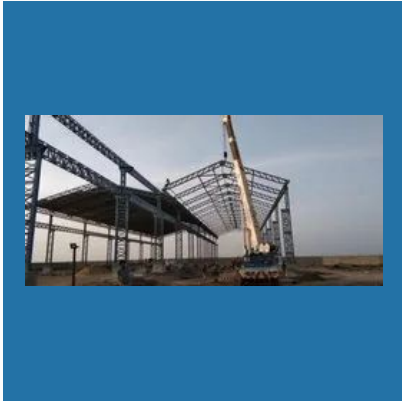
Tin Shed Fabrication
